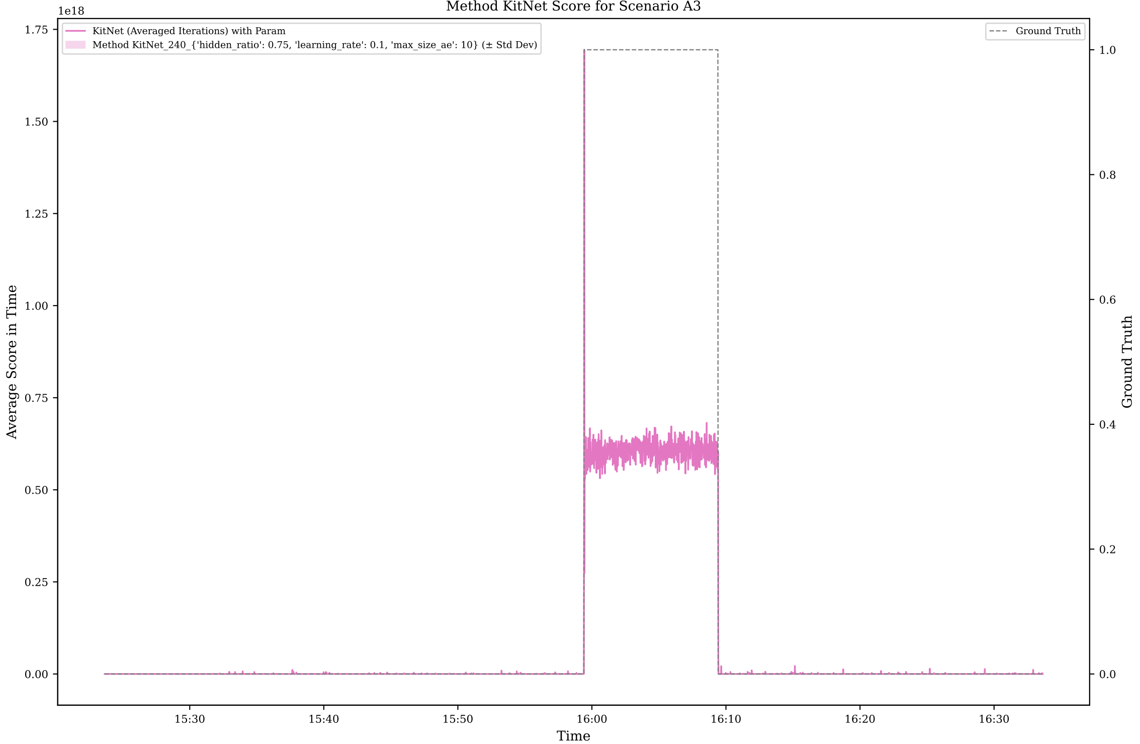
Method KitNet Score for Scenario A3
